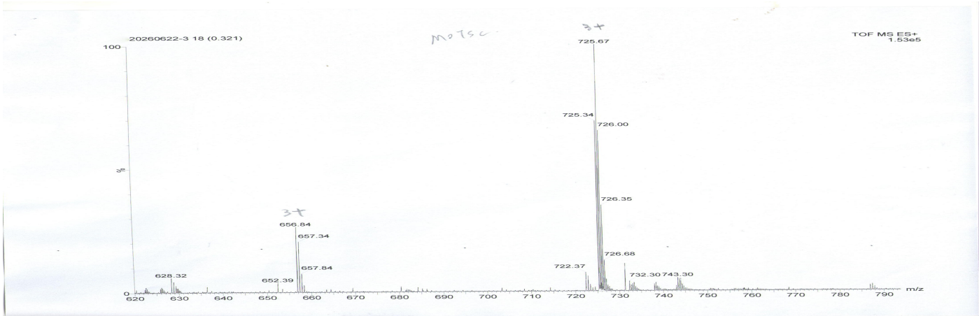
Mass Spectrum (ESI-MS)
